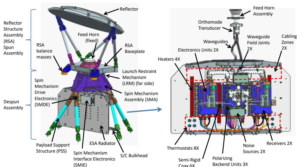
Figure 2-1. CAD representation of the COWVR instrument.
