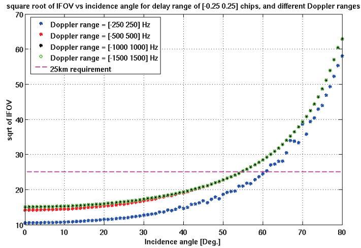
Figure B3. illustration of curves of square root of IFOV versus incidence angle, for a fixed delay range of [-0.25 0.25] chips, and different Doppler ranges. The dashed magenta line shows the 25 km requirement.
