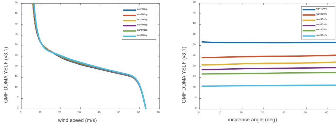
Fig. 32. YSLF GMF of \sigma_0 (DDMA) versus wind speed at different incidence angles (left) and versus incidence angle at different wind speeds (right).
