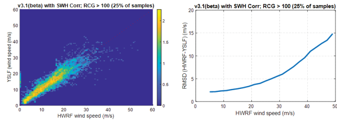
Figure A4. L2 YSLF wind speed vs. HWRF for subset of 2018 matchup population with RCG > 100.
