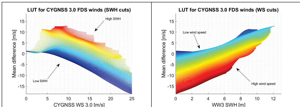
Fig. 34. Correcting LUT cuts: (left) SWH cuts and (right) WS cuts.
