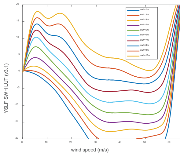
Fig. 35. Bias correction LUT for YSLF wind speed retrieval as a function of wind speed for different values of significant wave height.
