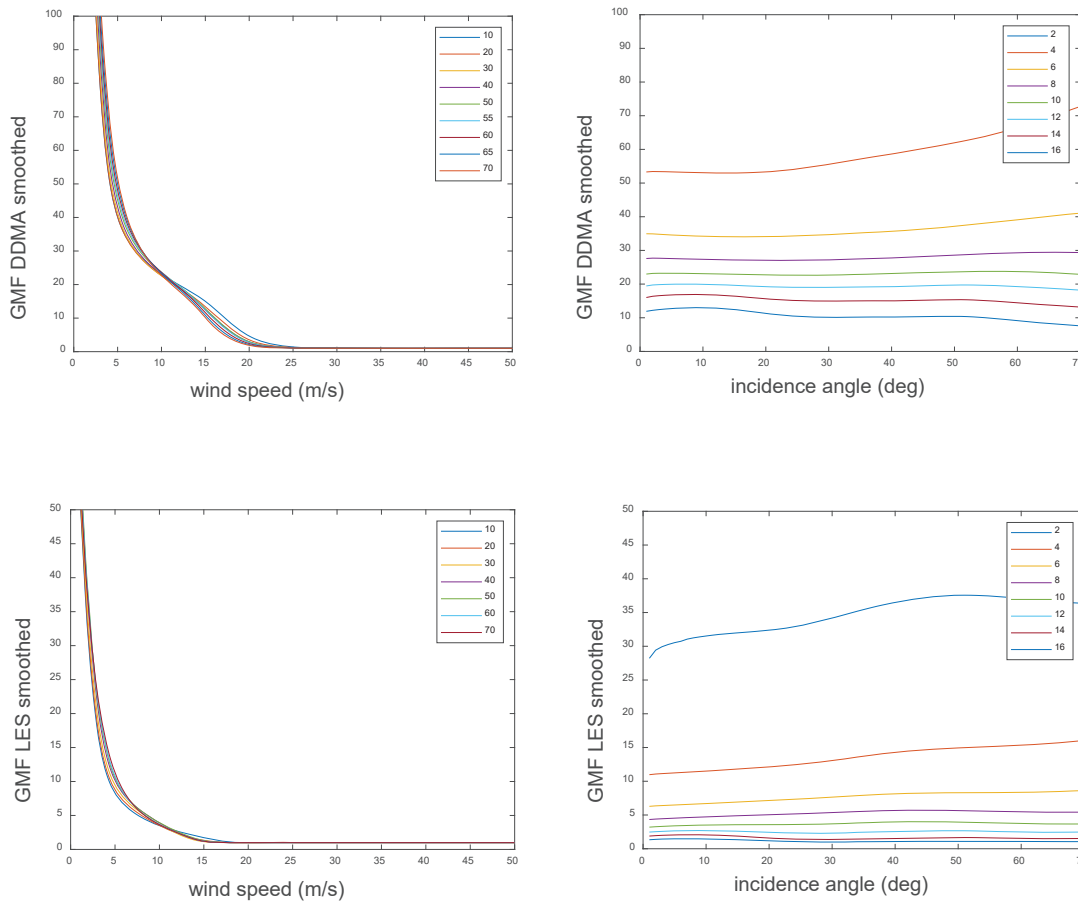
Figure 6. FDS GMFs for the two Level 1 observables, \sigma_o or DDMA (top) and LES (bottom). The GMFs are plotted as a function of wind speed for different incidence angles (left) and as a function of incidence angle for different wind speeds (right).
