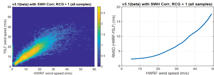
Figure A3. L2 YSLF wind speed vs. HWRF for complete 2018 matchup population.
