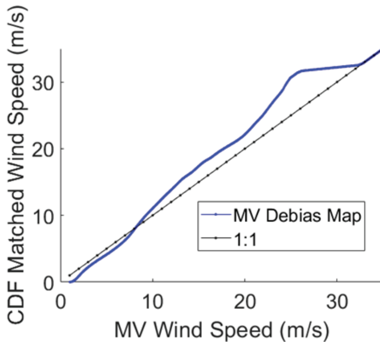
Figure B5. Significant wave height corrected MV wind debiasing map used to match the global probability distribution of CYGNSS L2 fully developed seas minimum variance wind speeds to those of the ERA5 reanalysis numerical weather prediction product. This example is for the starboard antenna of FM1 and GPS SVN 63. Maps for other CYGNSS antennas and GPS SVNs are similar.
