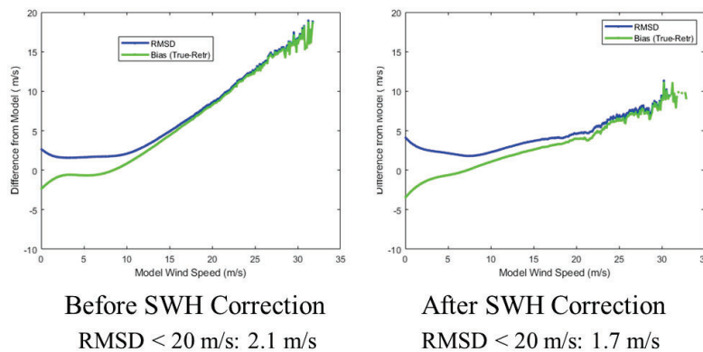
Fig. A2. FDS Minimum Variance (MV) wind speed retrieval bias and RMSD before (left) and after (right) SWH-dependent bias correction vs ERA5 wind speed.
