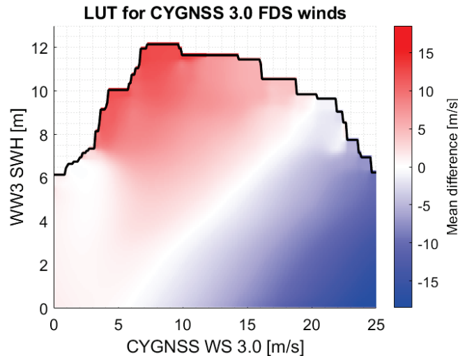
Fig. 33. Correcting LUT for v3.0 FDS winds.
