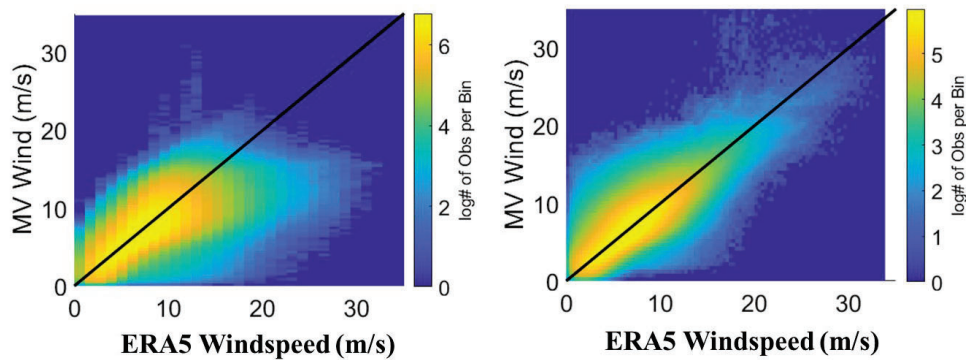
Fig. A1. FDS Minimum Variance (MV) wind speed retrieval scatterplots before (left) and after (right) SWH-dependent bias correction vs ERA5 wind speed.
