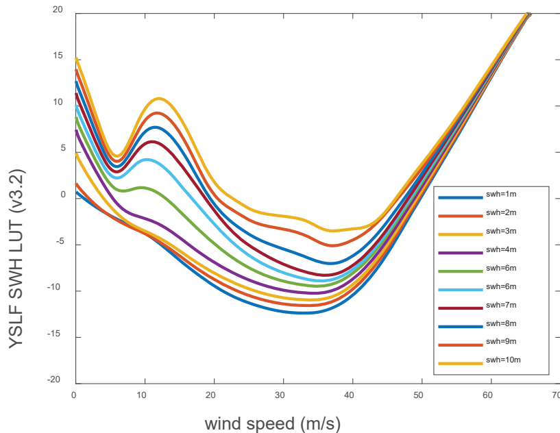
Fig. 37. Bias correction LUT for YSLF wind speed retrieval as a function of wind speed for different values of significant wave height.
