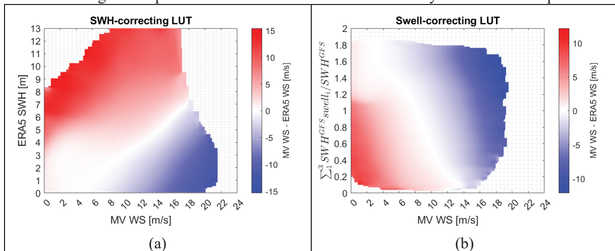
Fig. 34. SWH-correcting LUT (left) and swell-correcting LUT (right) for v3.2 FDS MV winds.
