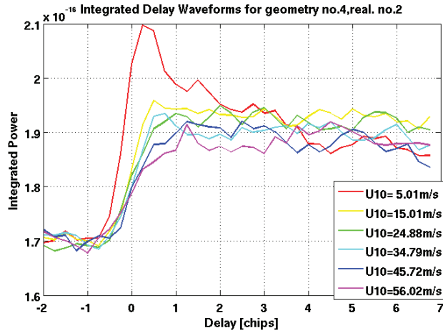
Figure 29. Integrated Delay Waveforms computed from DDMs simulated using different wind speeds.
