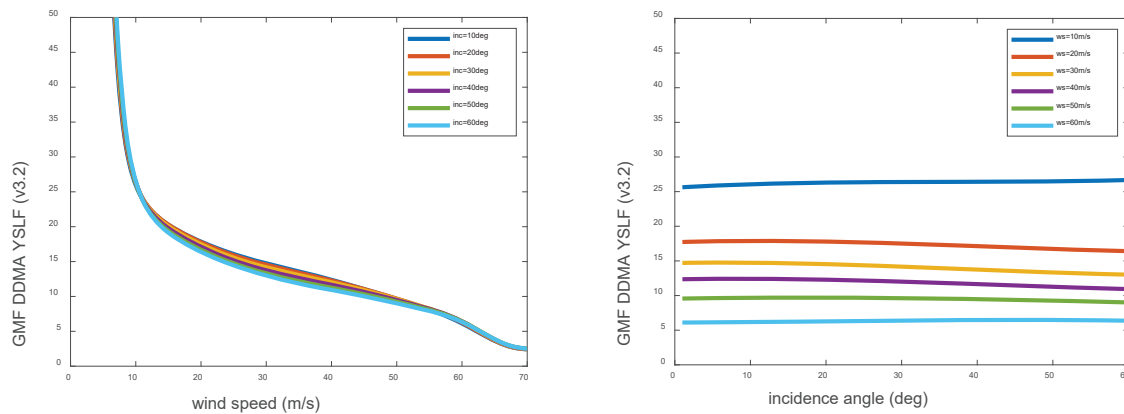
Fig. 33. YSLF GMF of \sigma_o (DDMA) versus wind speed at different incidence angles (left) and versus incidence angle at different wind speeds (right).
