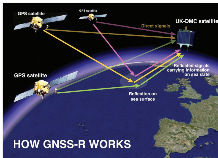
Figure 2. Measurement principle of GPS-Reflectometry over the ocean.
