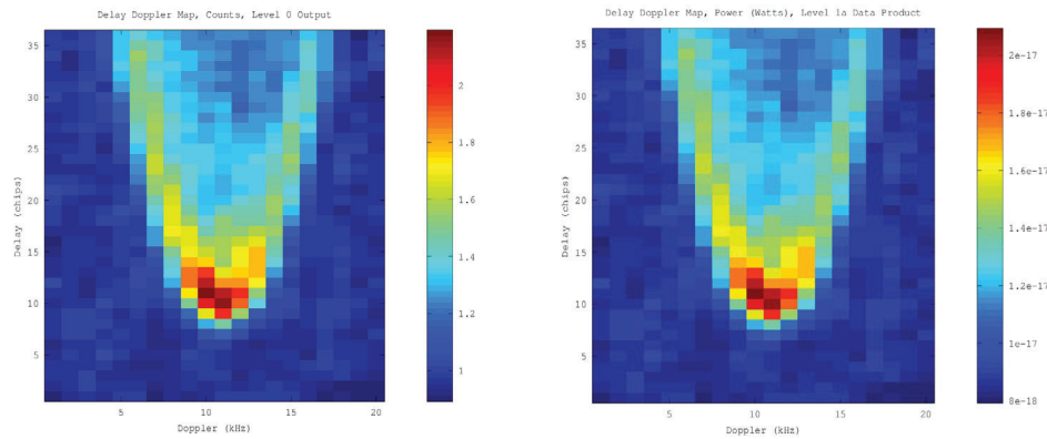
Figure 8. (left) raw Level 0 DDM in uncalibrated counts. (right) Level 1a calibrated DDM in units of Watts. DDMs generated by the CYGNSS End-to-End Simulator. Note the different magnitude scales before and after the Level 1a calibration.
