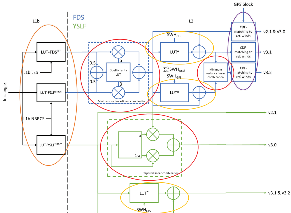
Figure 26. Signal flow diagram for the generation of L2 SDR wind speed.
