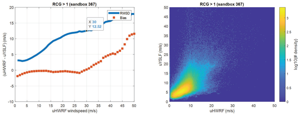
Figure A2. L2 YSLF wind speed vs. HWRF for complete 2018, 2020-2022 matchup population.
