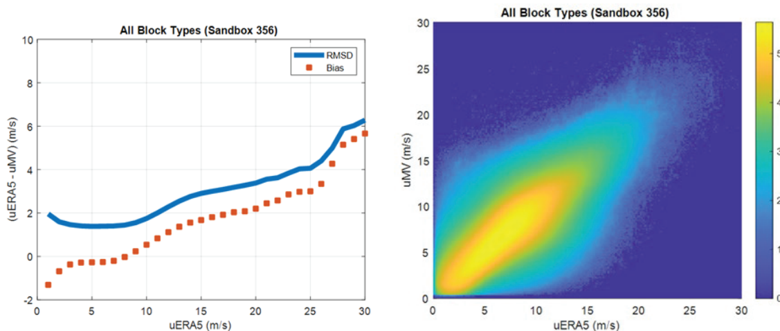
Fig. A1. FDS Minimum Variance (MV) wind speed RMSD and Bias and scatterplot vs ERA5 wind speed. The log of the number density of samples in each (windXwind) bin is shown.
