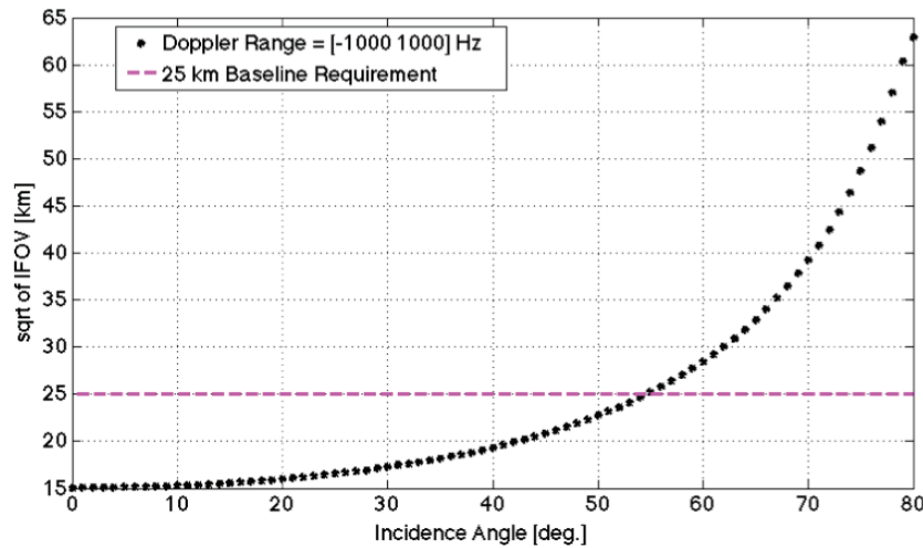
Figure 30. square root of Instantaneous Field of View (IFOV) versus incidence angle, for the DD window spanning -0.25 chip to 0.25 chip, and -1 kHz to 1 kHz (black dots), along with the requirements for the CYGNSS mission (dashed magenta line).
