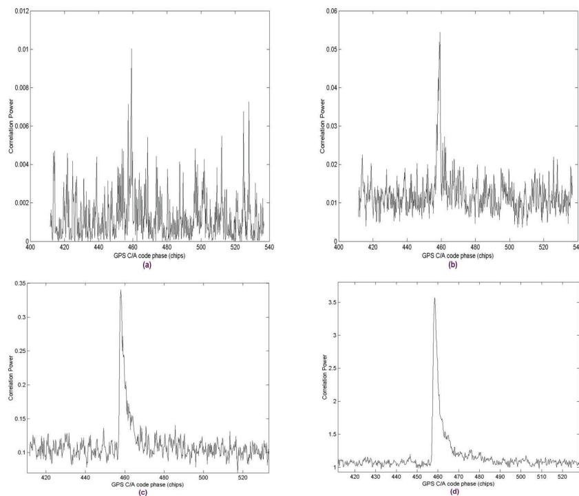
Figure 11. Examples of 1-D delay waveforms [from Gleason, 2006]
