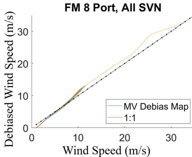
Figure B5. Significant wave height corrected MV wind debiasing map used to match the global probability distribution of CYGNSS L2 fully developed seas minimum variance wind speeds to those of the ERA5 reanalysis numerical weather prediction product. This example is for the port antenna of FM8 all SVNs (various colors). Maps for other CYGNSS antennas are similar.
