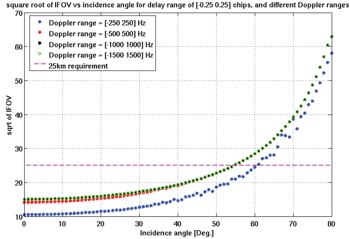
Figure B3. illustration of curves of square root of IFOV versus incidence angle, for a fixed delay range of [-0.25 0.25] chips, and different Doppler ranges. The dashed magenta line shows the 25 km requirement.
