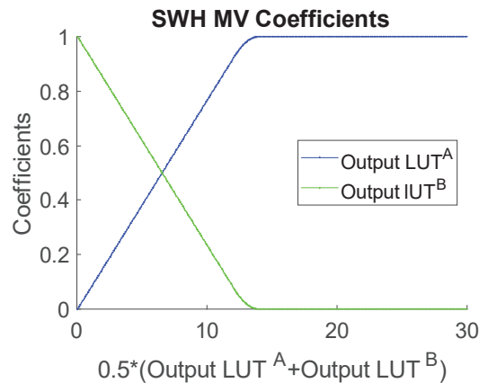
Fig. 36. Minimum variance coefficients used to combine corrections from the SWH correcting LUT A and swell correcting LUT B.
