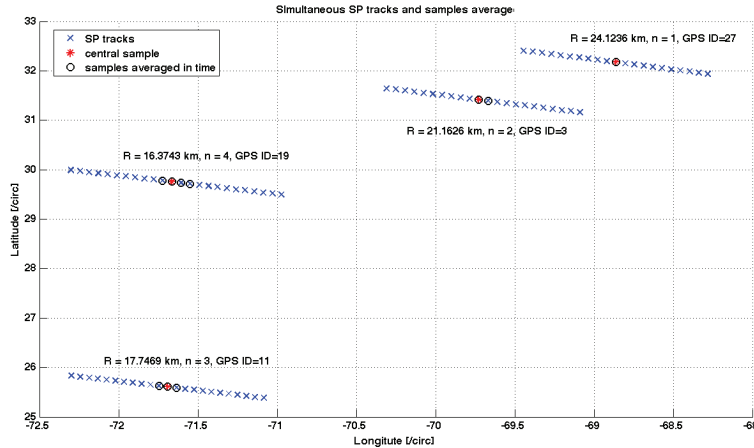
Figure 31. An illustration of how the Time Averaging (TA) algorithm works, for four simultaneous SP tracks acquired by a single CYGNSS observatory.
