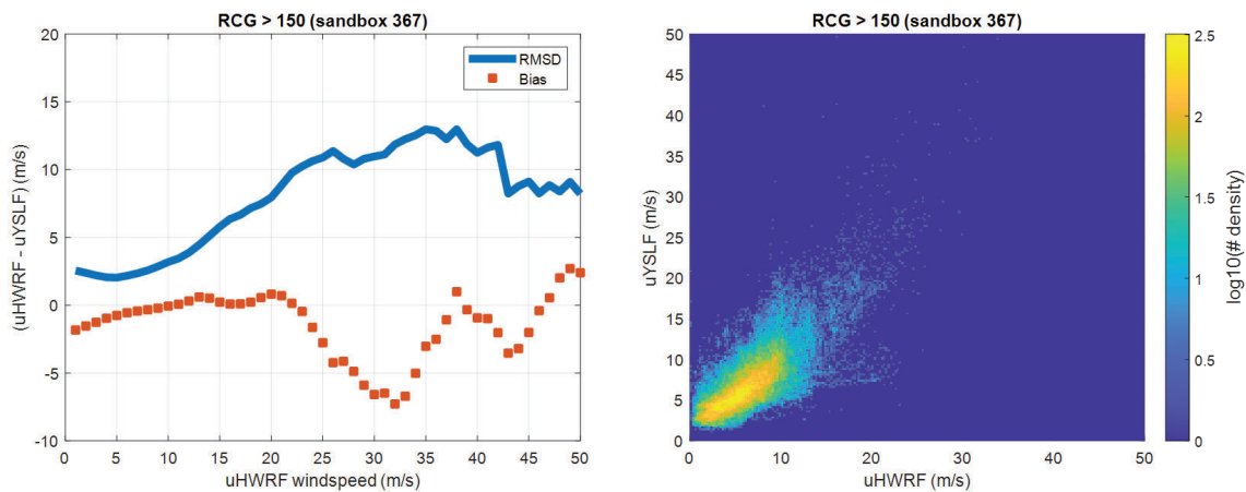
Figure A3. L2 YSLF wind speed vs. HWRF for subset of 2018, 2020-2022 matchup population with RCG > 150.
