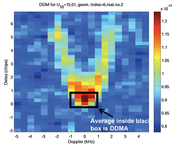
Figure 28. A simulated DDM and the DDM area where the DDMA is calculated.
