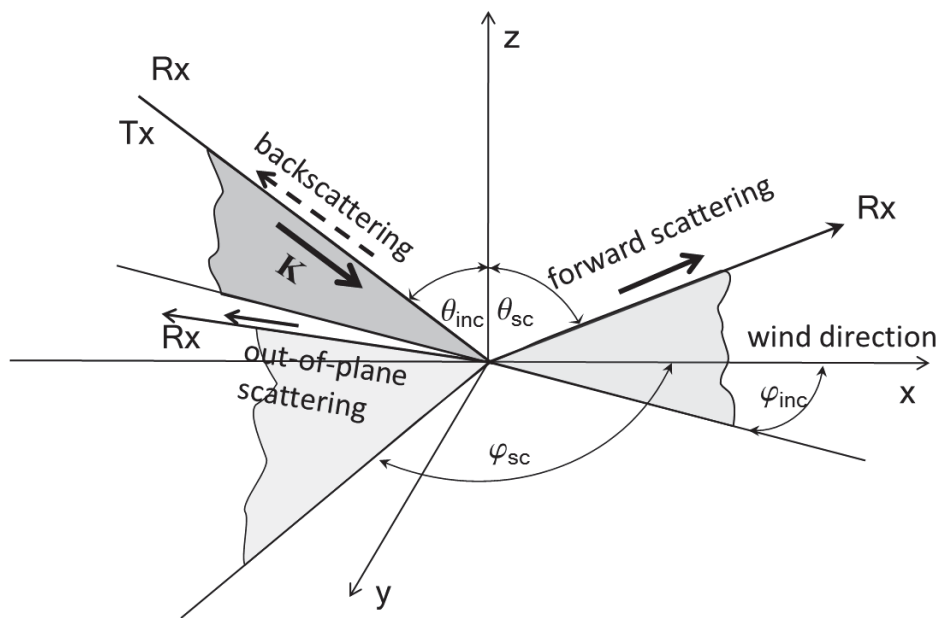
Figure 15. Geometry of the scattering problem for SSA.
