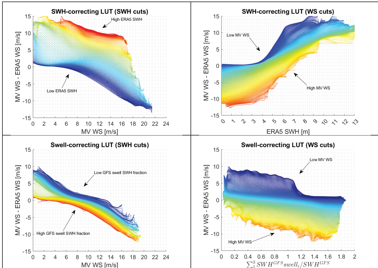
Fig. 35. Cuts for (top) SWH correcting LUT and (bottom) swell-correcting LUT.
