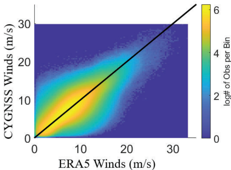
Figure B6. Scatter plot of collocated ERA5 and CYGNSS FDS winds with SWH correction and debiasing applied.
