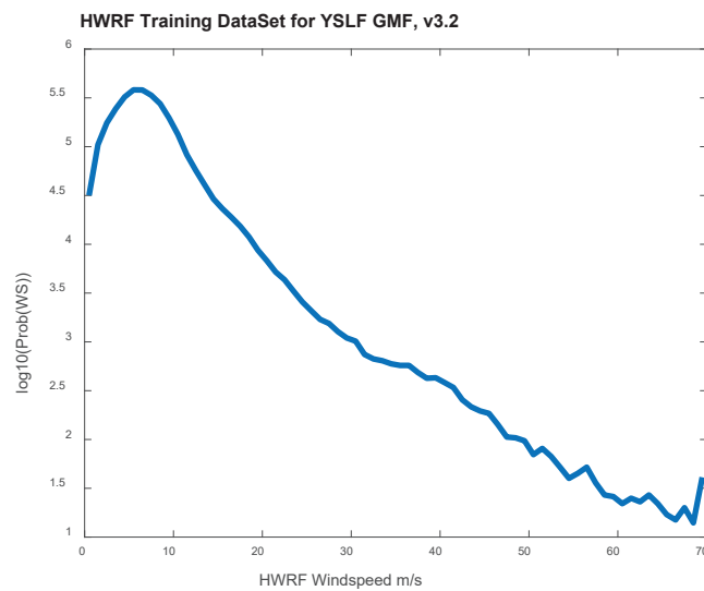
Figure 27. Histogram of wind speeds in the matchup population used to train the YSLF GMF.
