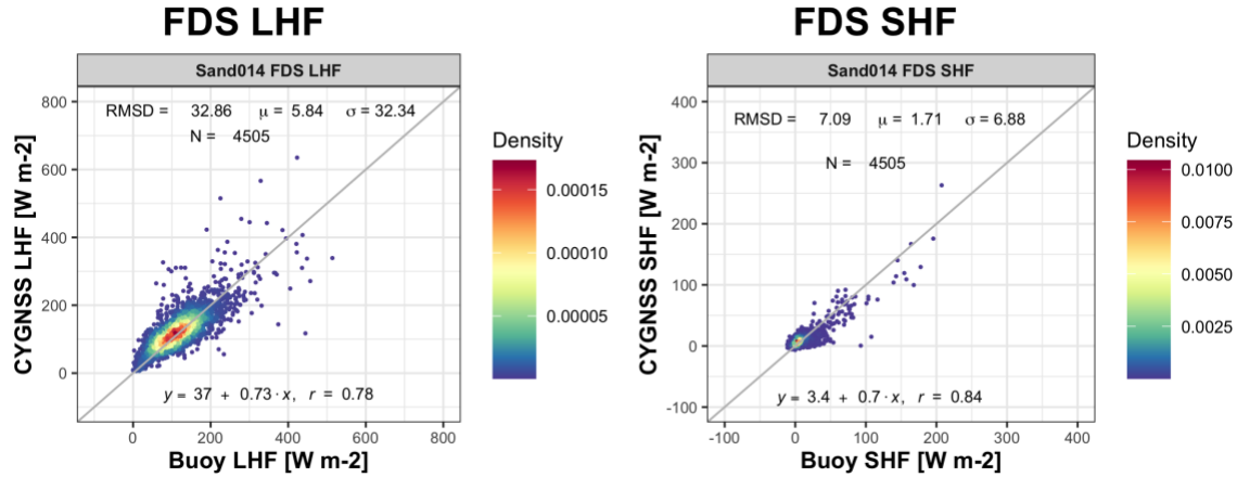
Figure 5: CYGNSS surface heat flux comparisons (y-axis) compared to flux estimates from buoys (x-axis). Left: Latent heat flux. Right: Sensible heat flux.
