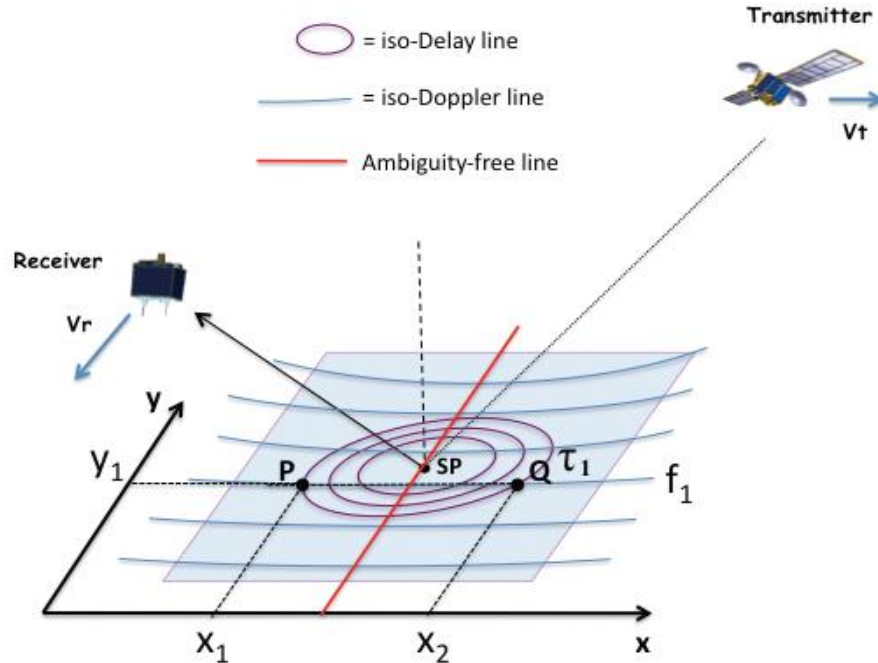
Figure 2: GPS signal propagation and scattering geometries for ocean surface bistatic quasi-specular scatterometry. Reused from Clarizia & Ruf (2016), © 2016 IEEE.
