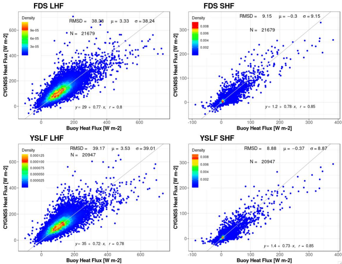
Figure 5: CYGNSS surface heat flux comparisons (y-axis) compared to flux estimates from buoys (x-axis). Top row: CYGNSS LHF and SHF estimates using the FDS wind speed product. Bottom Row: CYGNSS LHF and SHF estimates using the YSLF wind speed product. Left: Latent heat flux. Right: Sensible heat flux.
