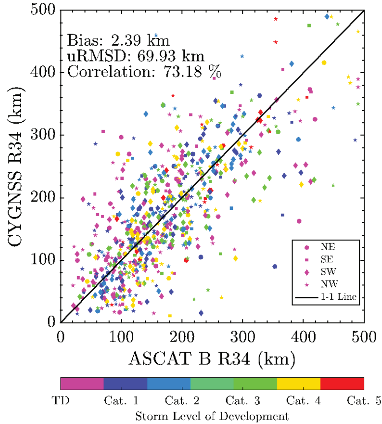
Fig. 5. R34 retrieval comparisons to ASCAT-B using a CYGNSS data record spanning all co-located storms over the period 2020-2023. Storm intensity indicated by color. Storm quadrant indicated by marker symbol. Correlation estimated to be 73.18%.
