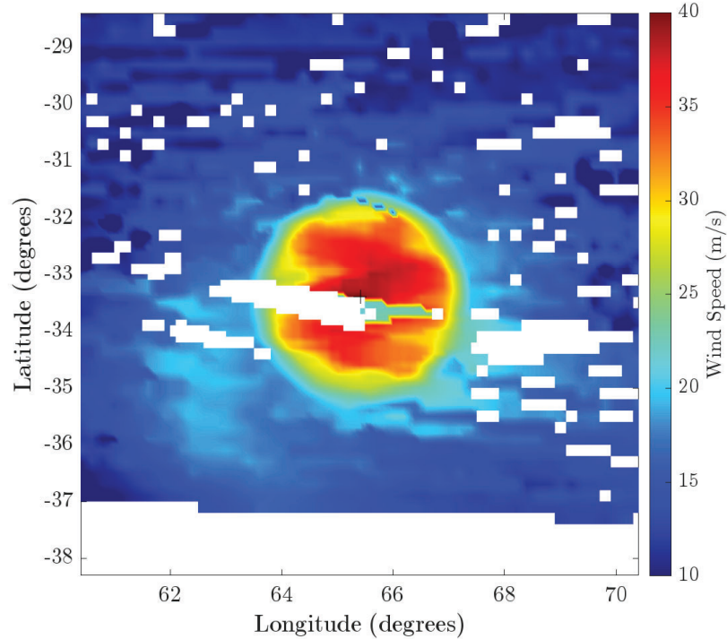
Fig. 2. Example CYGNSS L3 MRG wind field from TC Calvinia, Jan 1, 2020 0600Z.
