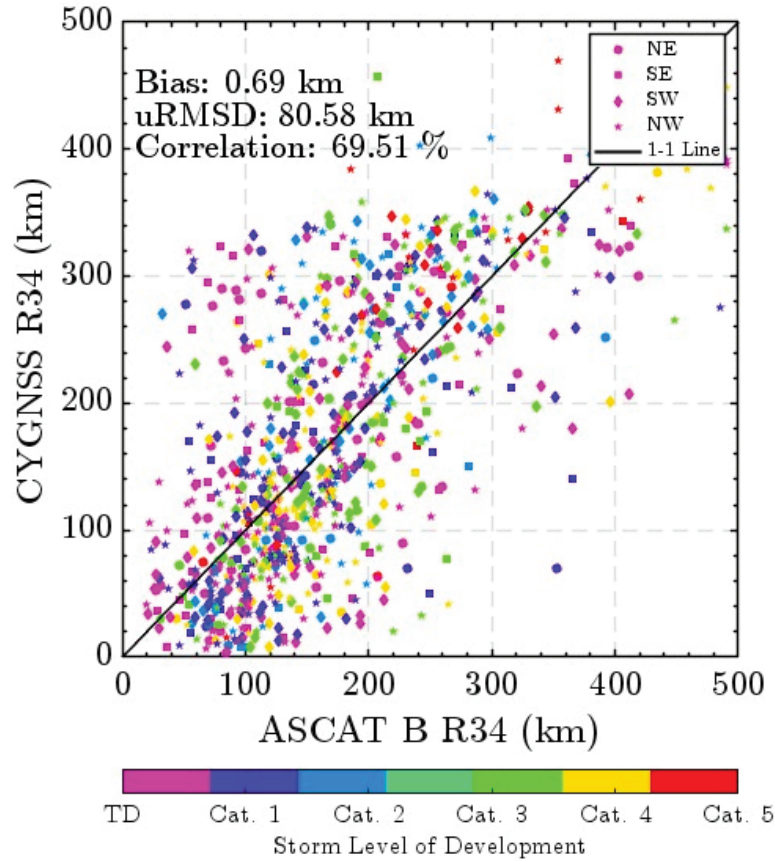
Fig. 5. R34 retrieval comparisons to ASCAT-B using a CYGNSS data record spanning all co-located storms over the period 2020-2024. Storm intensity indicated by color. Storm quadrant indicated by marker symbol. Correlation estimated to be 69.51%.
