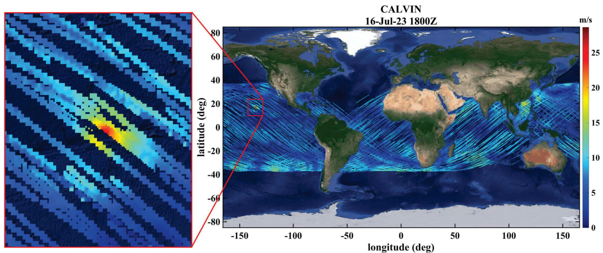
Fig. 6. Example L3 MRG wind field from Hurricane Calvin at reporting time July 16, 2023 1800Z. Left: Wind field in the vicinity of the TC (corresponding to red box on the right figure);
