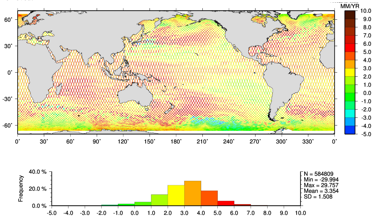
Figure 20: Global mean sea level variations estimated as in Figure 22 with annual and semi-annual signal removed.
