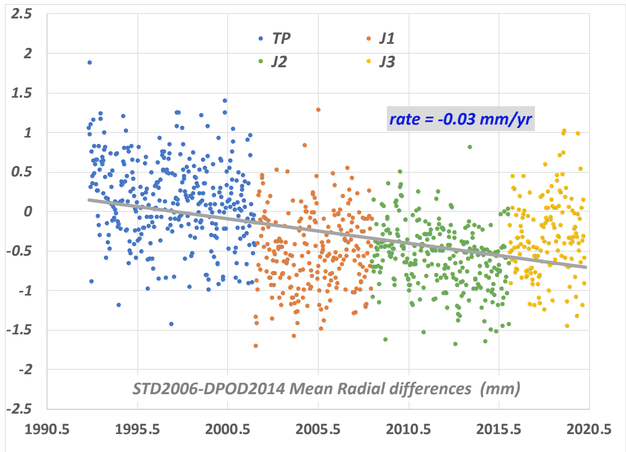
Figure 4b: Mean radial std2006-dpod2014 orbit differences/cycle over water.
