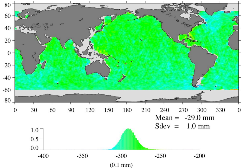
Figure 14: v5.0 Jason-3 minus Jason-2 inter-mission bias is estimated from averaged SSH collinear residuals during Jason-3 verification phase. Color scale is +/- 1cm about estimated mean.
