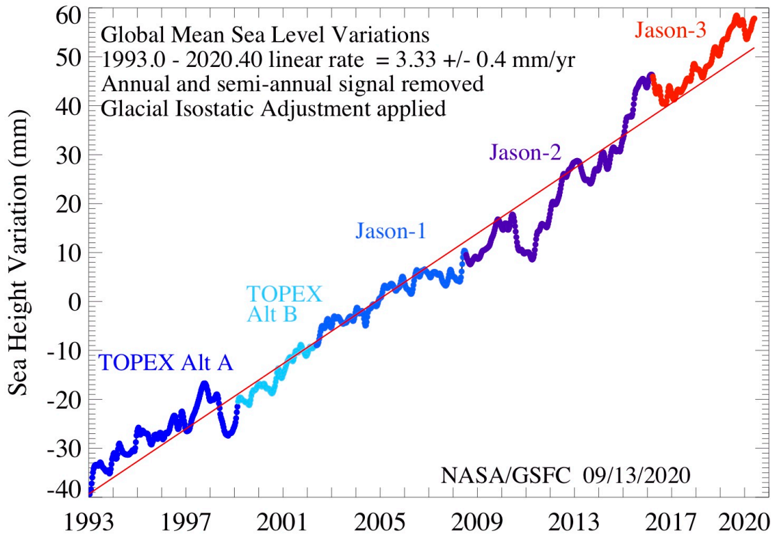
Figure 20: Global mean sea level variations estimated as in Figure 22 with annual and semi-annual signal removed.
