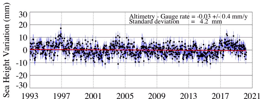
Figure 18: Resultant per cycle comparisons of altimeter derived v5.0 SSH variations with height variations from 64-site tide gauge network after application of inter-mission biases to form a single adjusted SSH Climate Data Record.
