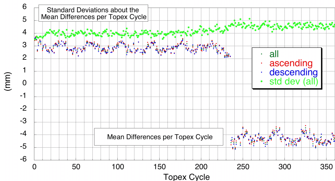
Figure 11: Mean differences of sea surface height between heights based on parametric versus non-parametric sea state bias solutions reveals separate biases (Chambers et al., 2003) for TOPEX Side A (cycles 1-235) and for Side B (cycles 236-364).
