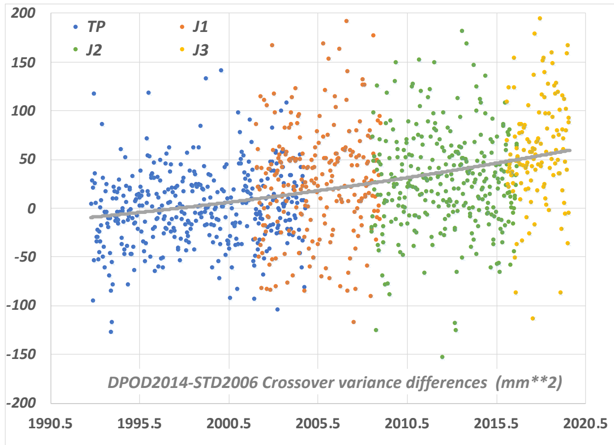
Figure 4a: std2006 radial orbit accuracy relative to dpod2014 using independent crossover data. Positive values indicate improvement derived from std2006.
