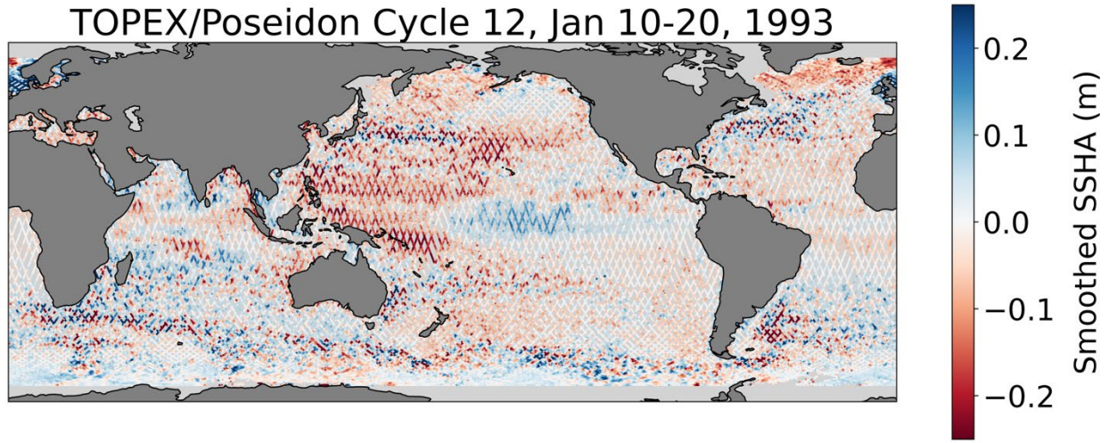
Figure 2: Map of the smoothed SSHA from 10 daily files from January 10 to January 20, 1993.
