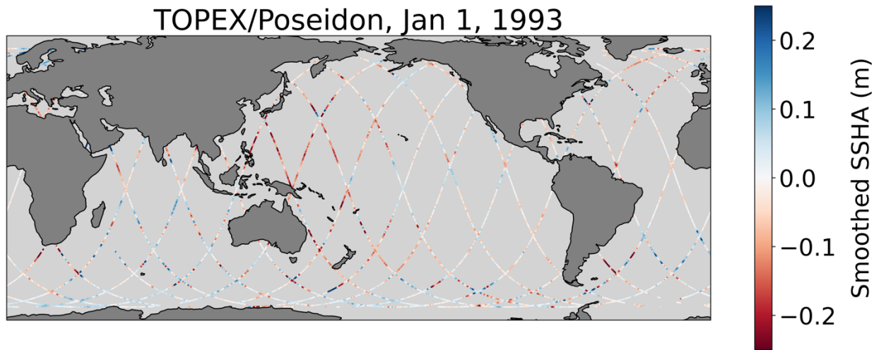
Figure 3: Map of the smoothed SSHA from 1 daily file on January 1, 1993.
