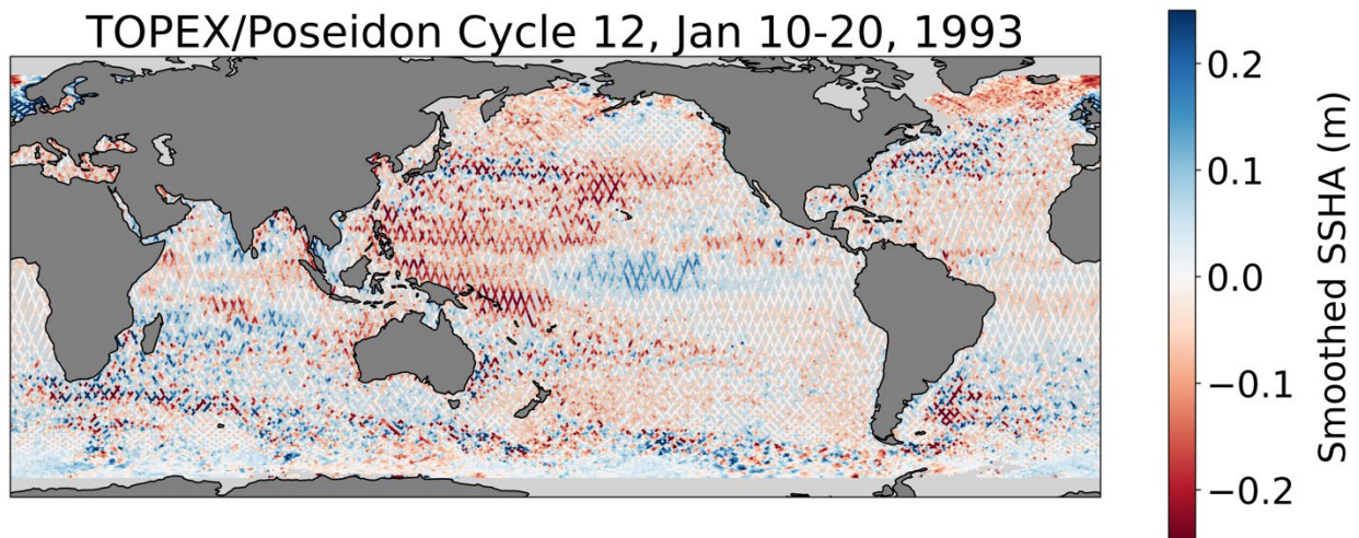
Figure 8: Map of the smoothed SSHA from 10 daily files from January 10 to January 20, 1993.
