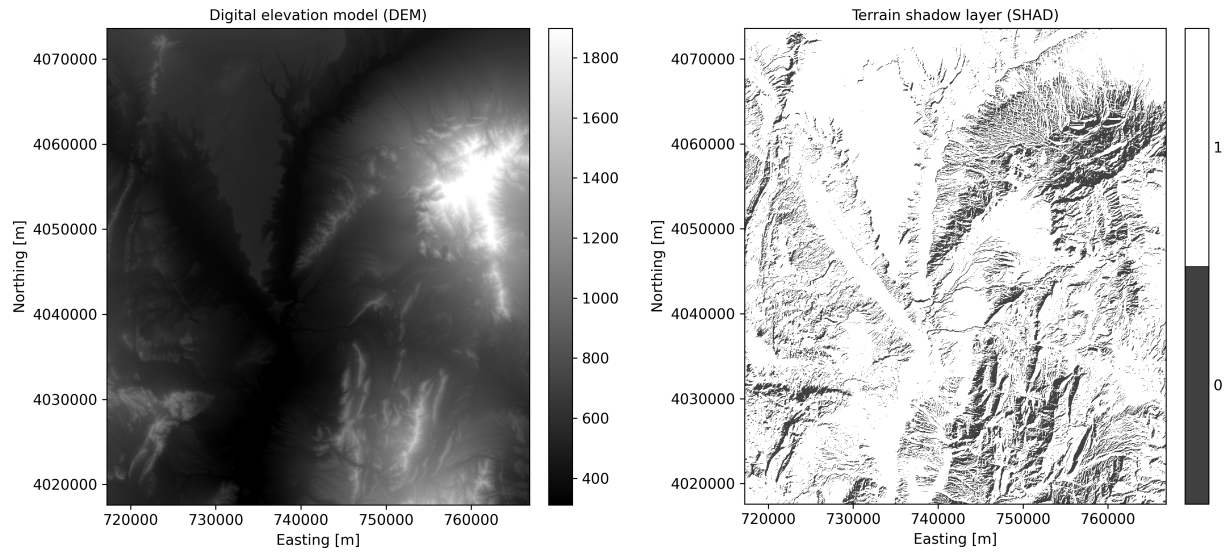
Figure 5-3. Digital elevation model DEM (left) and Terrain shadow layer SHAD (right).
