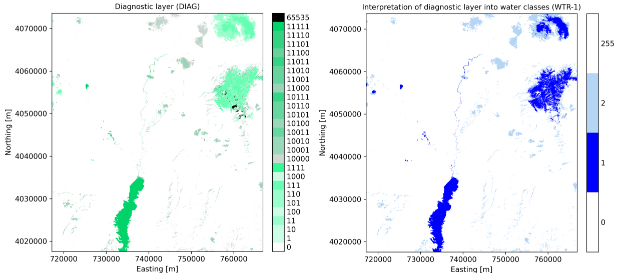
Figure 5-2. Diagnostic layer DIAG (left) and interpretation of diagnostic layer into water classes WTR-1 (right).
