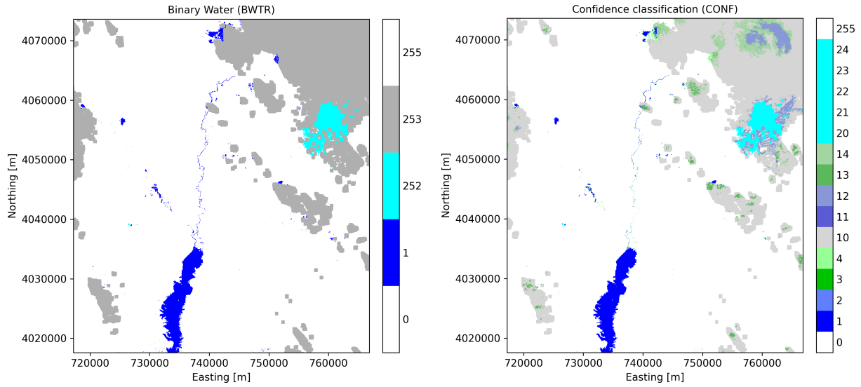
Figure 5-6. Binary water layer BWTR (left) and confidence layer CONF (right).
