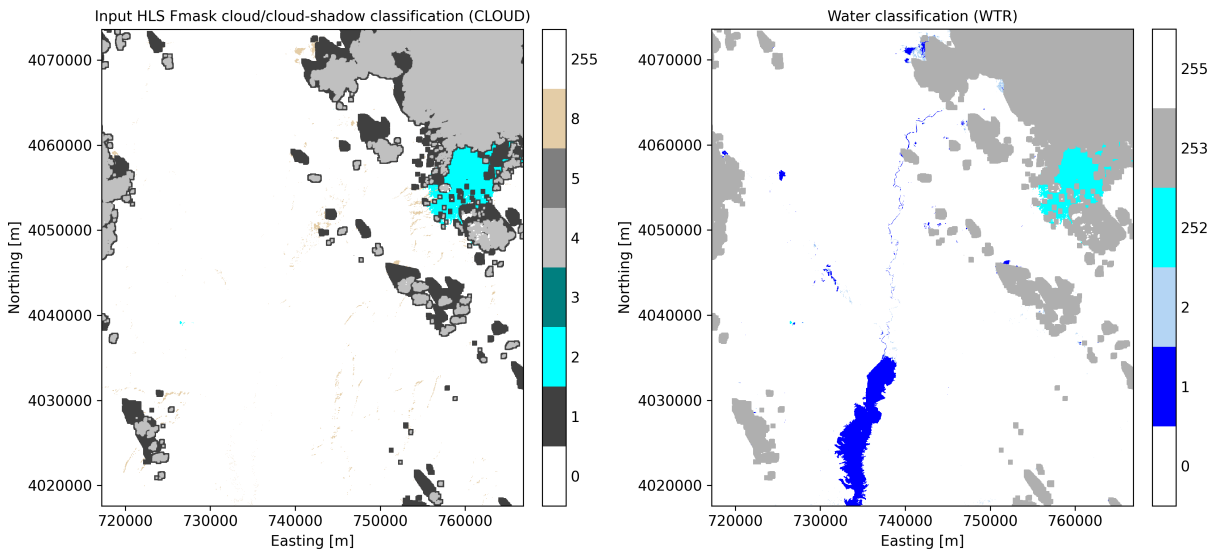
Figure 5-5. Input HLS Fmask cloud/cloud-shadow/water classification CLOUD (left) and the interpreted water classification WTR (right).
