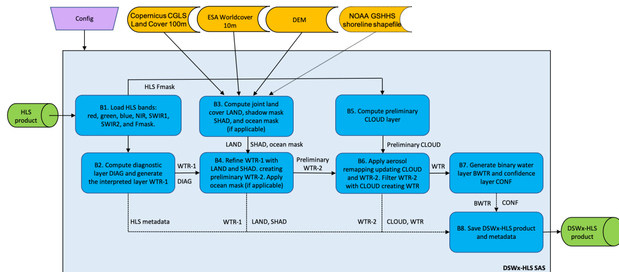
Figure 2-1. OPERA DSWx-HLS workflow diagram.
