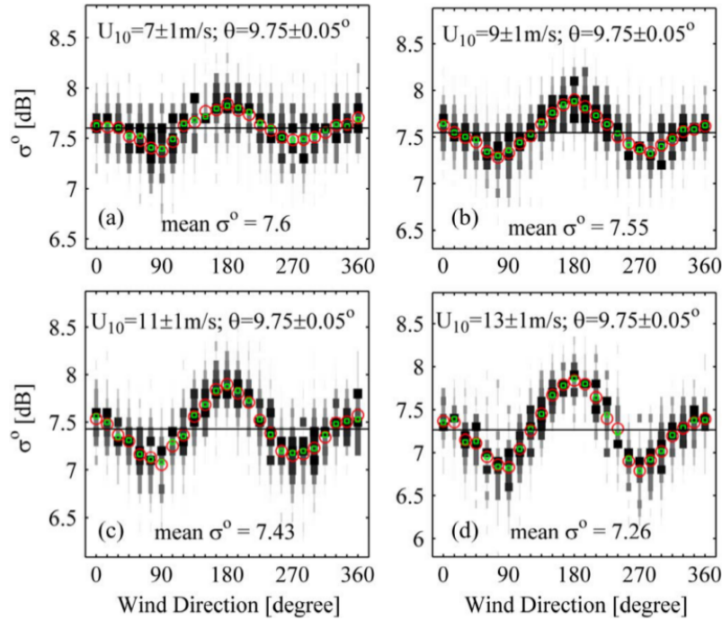
Figure 33: Box plot of \tilde{\sigma}^0 measured by Tropical Rainfall Measuring Mission precipitation Radar in each 15° azimuthal interval. Widths and gray levels of boxes show the distribution of data. Mean and median are shown as red circles and green squares, respectively. Extracted from [R3].
