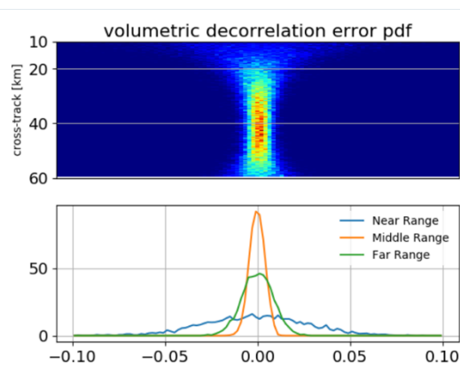
Figure 24: Probability density function for volumetric correlation (SWH=2m)
