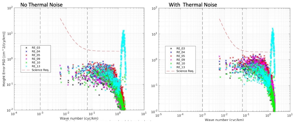
Figure 10: Unsmoothed error spectra from the 200 km long simulations with 2 m SWH (left panel: no thermal noise, right panel: with thermal noise).
