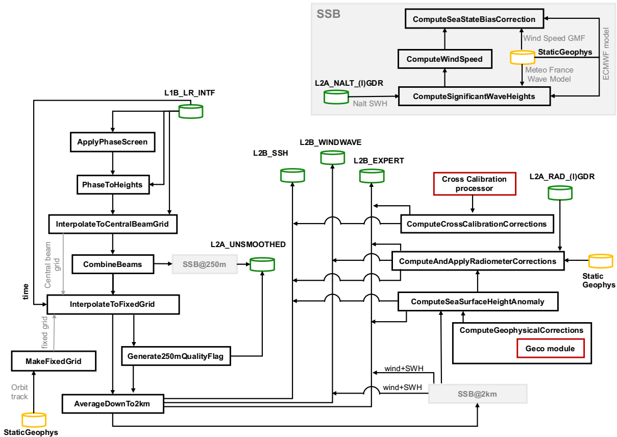
Figure 2: Interface Diagram.
