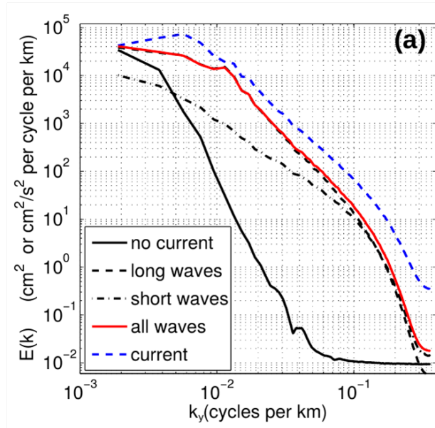
Figure 26: From [13]. The black and red solid lines ( cm^2/(cycles/km) ) and the dashed blue line ( cm^2/s^2/(cycles/km) ) are respectively the spectra of Figure 25-(c), Figure 25-(b) and Figure 25-(a). The SWH spectrum with currents follows the current spectrum (in k^{-2.5} ). Note that at periods < (g \cdot 2\pi \cdot [k_y \times 10^{-3}])^{-1/2} = 6 s, the short waves exceed the long waves.
